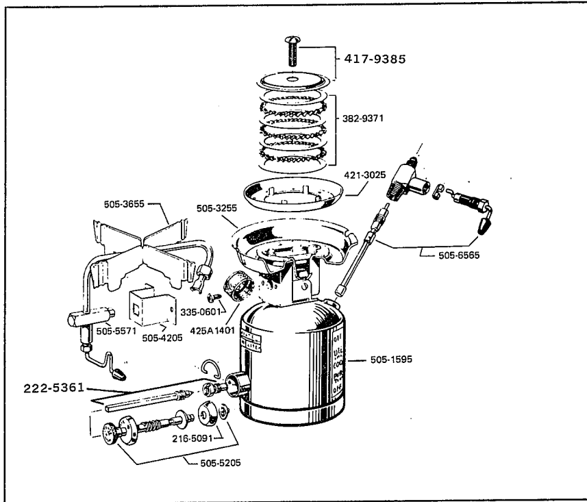
MODEL 505 SINGLE BURNER – CAMP STOVE
